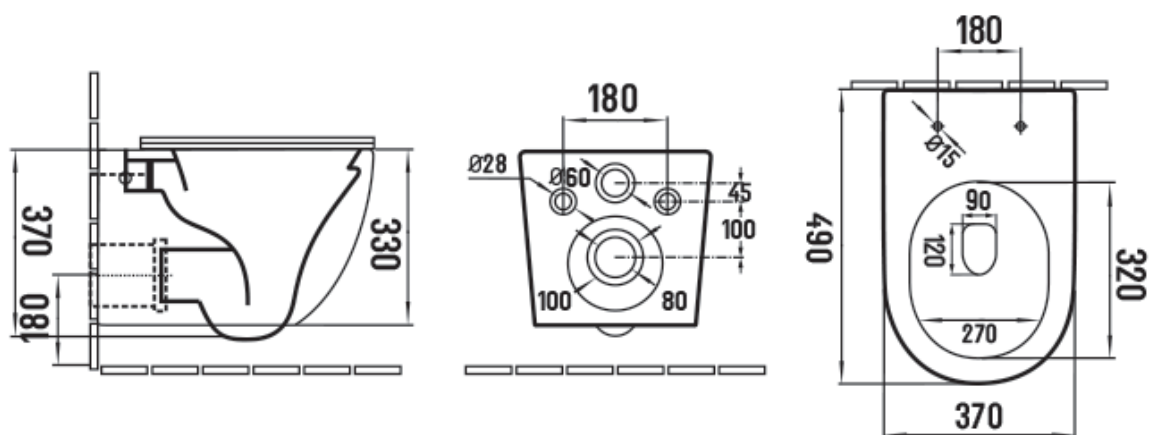
Wall-hung toilet Size:490x370x370mm P-trap:180mm Roughing-in
